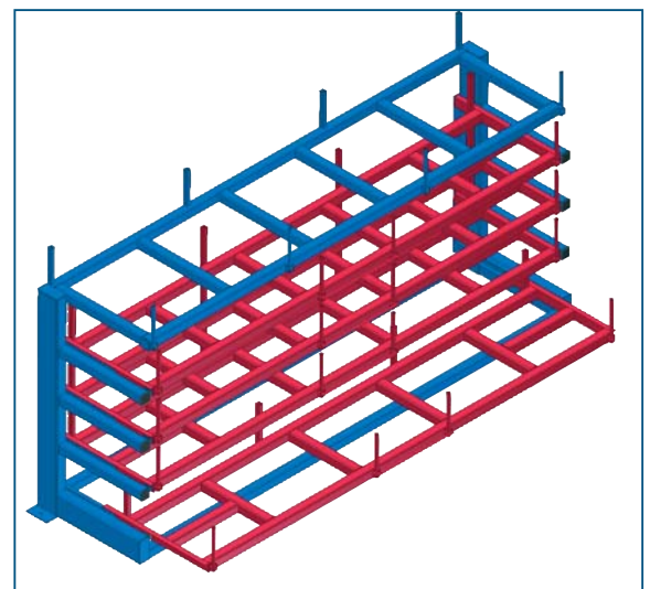
Type SRL 4 + 1
